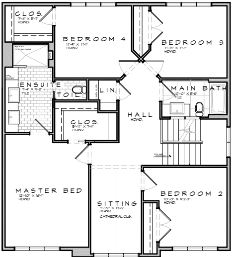
SECOND FLOOR PLAN 1343 SQFT.
